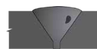
37 Slag Inclusion in Single Vee (weld groove area) UT, RT
