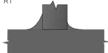
73 Uneven Leg Length in Fillet, VT
