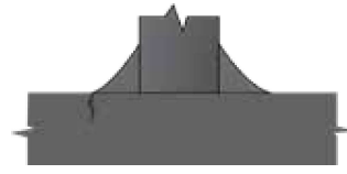
11 Toe Crack in Fillet MT/PT, UT
