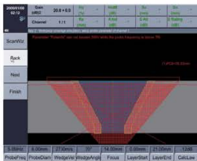
Beam Coverage Simulation
