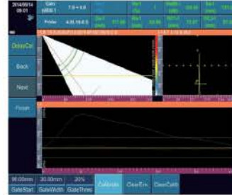
Delay Calibration
