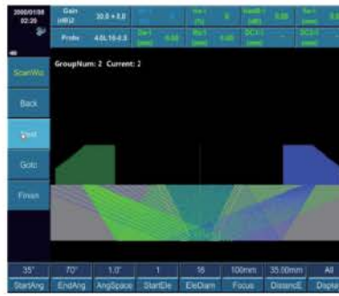
Beam Coverage Simulation (PA Groups)
