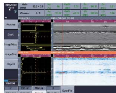
TOFD+Conventional UT to inspect the blind zone area
