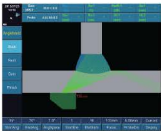
Flange Simulation
