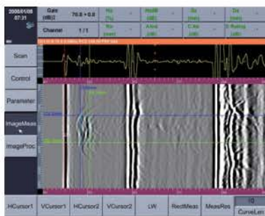
TOFD Measurement
