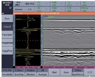
Horizontal TOFD image
