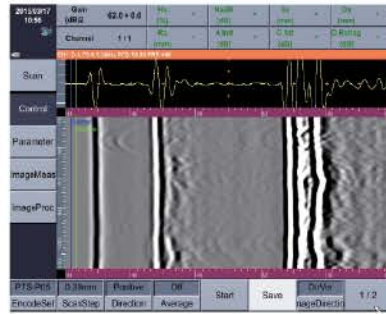
Longitudinal TOFD image
