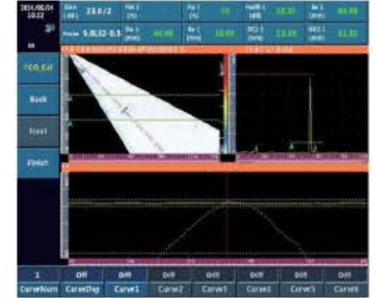
TCG Calibration
