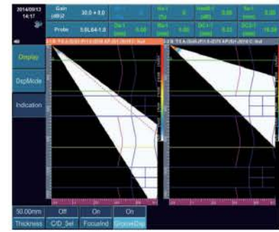
Flat Weld Groove
