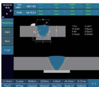
Y-weld with backing
