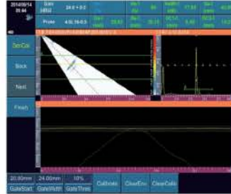
Sensitivity Calibration
