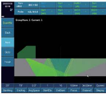
Beam Coverage Simulation(Single Probe)
